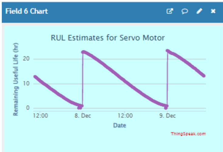
RUL Estimate Chart
